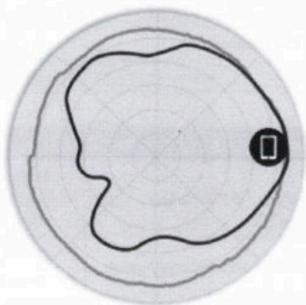
Figure 3. 5GHz Azimuth Antenna Patterns
