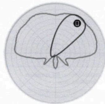
Figure 5. 5GHz Elevation Antenna Patterns
