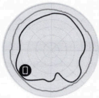
Figure 2. 2.4GHz Azimuth Antenna Patterns
